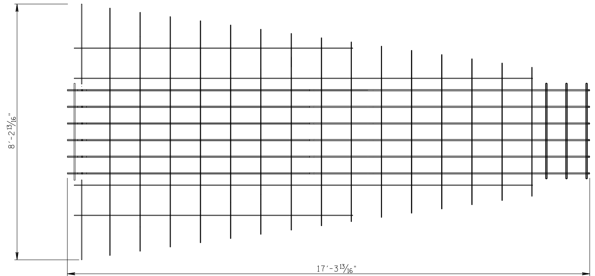
COMBINED MAT1 AND MAT2 (SHOWN WITHOUT BENDS)
